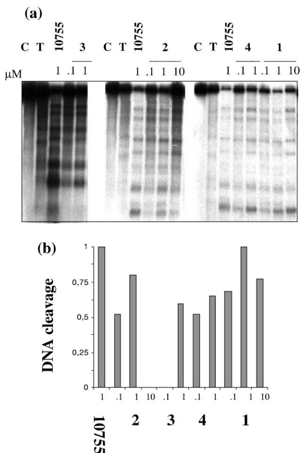
Figure 2. (a) Stimulation of topoisomerase II mediated DNA cleavage by the anthracycline analogues 1–4 and the reference compound MEN 10755. Lane C, control DNA; lane T, topoisomerase II alone. (b) Quantification of topoisomerase II dependent DNA cleavage stimulated by anthracycline analogues in SV40 DNA. DNA cleavage levels were determined at different sites with an analysis performed on a Macintosh computer using the public domain NIH Image program (developed at the US National Institute of Health and available on the internet at http://RSB.info.nih.gov/nih-image ). To normalize among different experiments, the stimulation factor of MEN 10755 at 1 M, which was included in all the gels, was used as an internal standard.
