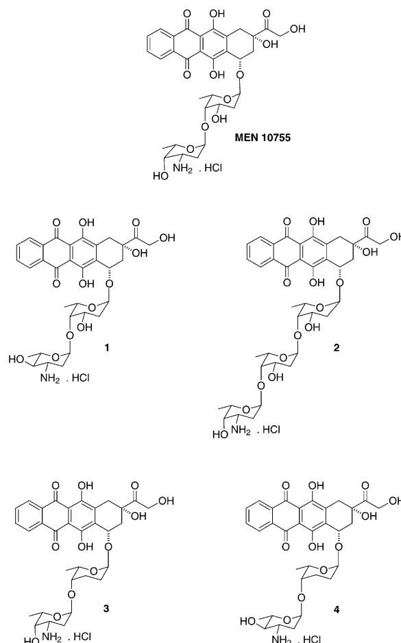
Figure 1. Molecular structures of MEN 10755 and oligosaccharide modified anthracyclines.
