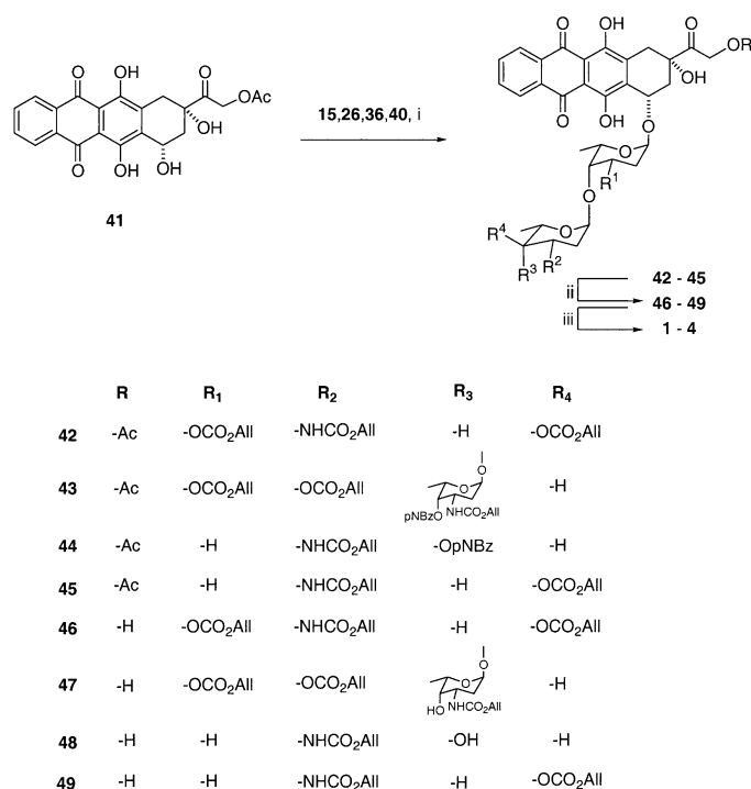
Scheme 3. (i) TMSOTf, CH 2 Cl 2 –Et 2 O, M.S. 4 Å, –20 °C, 2 h; (ii) 0.5 M K 2 CO 3 , MeOH–CH 2 Cl 2 , –10 °C, 1 h; (iii) (a) [(Ph 3 P) 4 ]Pd, Me 2 NTMS, TMSOAc, CH 2 Cl 2 , rt, dark, 0.5 h; (b) 0.001 M aq HCl.
