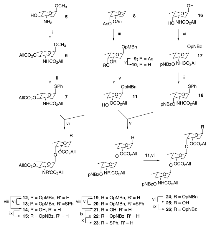
Scheme 1. (i) \text{AlI}(\text{OCOCl})_2 , py, \text{CH}_2\text{Cl}_2 , rt, 4 h; (ii) \text{PhSSiMe}_3 , \text{CF}_3\text{SO}_3\text{SiMe}_3 , \text{CH}_2\text{Cl}_2 , rt, 2 h; (iii) ( p -MeO) \text{C}_6\text{H}_4\text{CH}_2\text{OH} ( p -MBnOH), \text{Ph}_3\text{PBr} , \text{CH}_2\text{Cl}_2 , rt, 1 h; (iv) 1 N MeONa, MeOH, rt, 2 h; (v) (a) \text{Bu}_2\text{SnO} , toluene, reflux, 12 h; (b) \text{AlI}(\text{OCOCl})_2 , \text{Et}_3\text{N} , \text{CH}_2\text{Cl}_2 , -40^\circ\text{C} , 2 h; (vi) IDCP, (\text{CH}_2\text{Cl})_2\text{-Et}_2\text{O} , M.S. 4 Å, 10^\circ\text{C} , 2 h; (vii) \text{Ph}_3\text{P} , 1 h; (viii) \text{Ce}(\text{NH}_4)_2(\text{NO}_3)_6 , \text{CH}_3\text{CN-H}_2\text{O} , rt, 2 h; (ix) ( p - \text{NO}_2 ) \text{C}_6\text{H}_4\text{COCl} ( p -NBzCl), py, \text{CH}_2\text{Cl}_2 , 0^\circ\text{C} , 1 h; (x) \text{PhSSiMe}_3 , \text{CF}_3\text{SO}_3\text{SiMe}_3 , \text{CH}_2\text{Cl}_2 , 0^\circ\text{C} , 1 h; (xi) p -NBzCl, py, \text{CH}_2\text{Cl}_2 , rt, 1 h.
